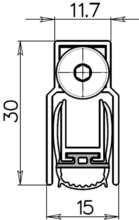
Fig. 5 Sectional drawing of floor seal
