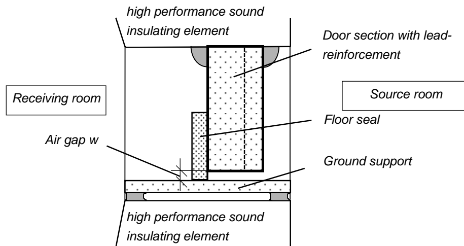
Vertical section
