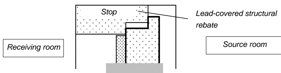
Horizontal section
