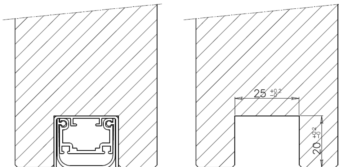
Figure 1 Sectional drawing 25/20 ASACA new
