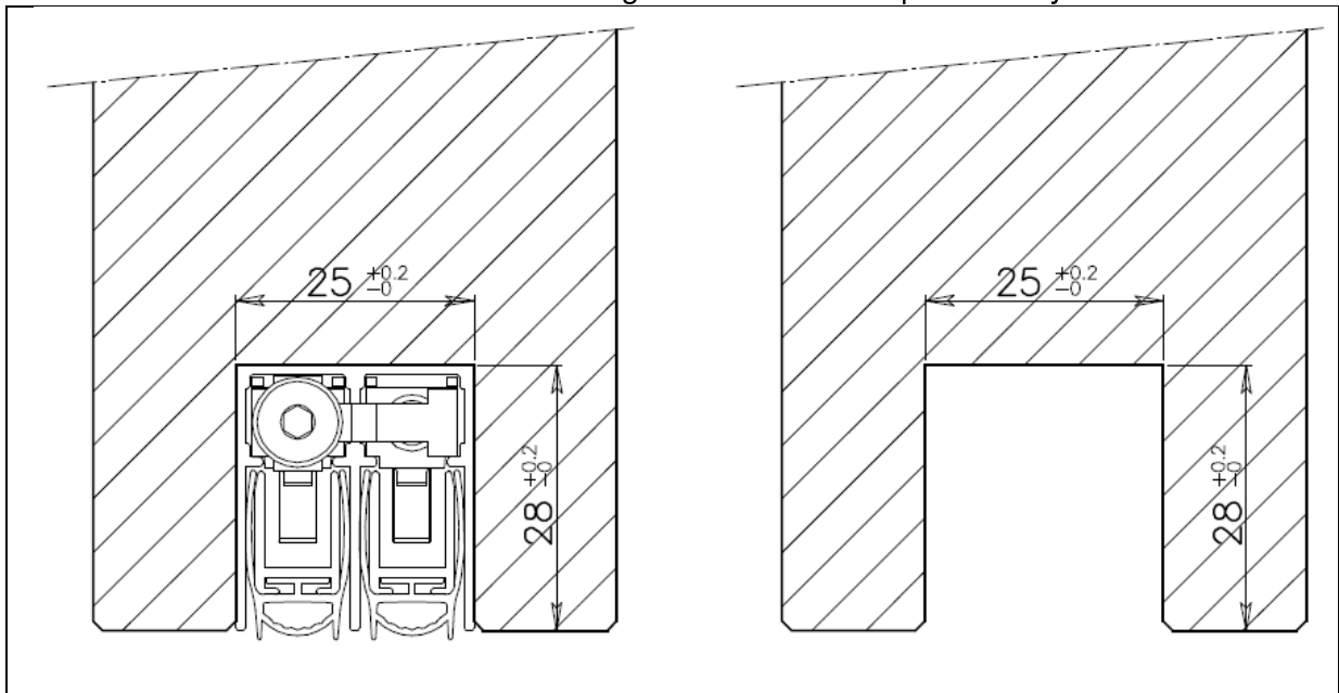
Figure 1 Sectional drawing 2x12.5/28 ASMPDP
