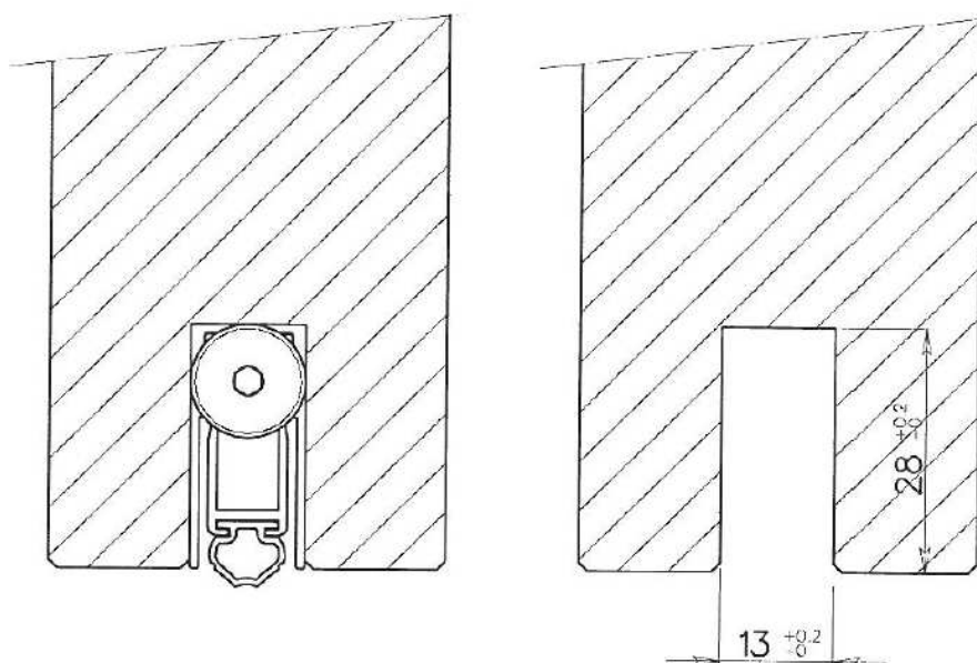
Figure 1 Sectional drawing 13/28 ASGSF-C
