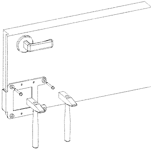
2B EASY-FIX
