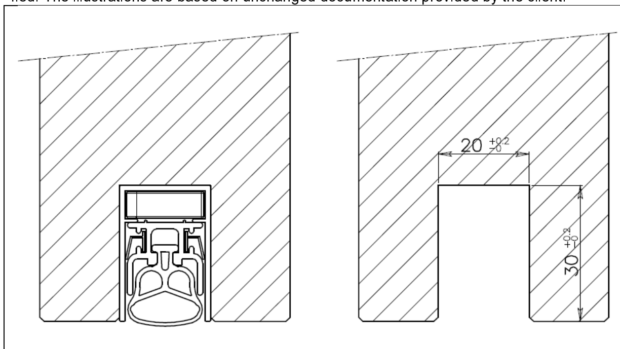
Figure 1 Sectional drawing 20/30 ASDB
